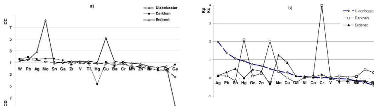
Figure 1. Background geochemical specialization of the region soils (a) and man-caused geochemical specialization of urban soils (b). Concentration (CC) or dispersion (CD) coefficients of metals in background soils were calculated compared to their global clarkes defined by A. P. Vinogradov (1962), coefficients Cc and Cd – relation to background soils.
