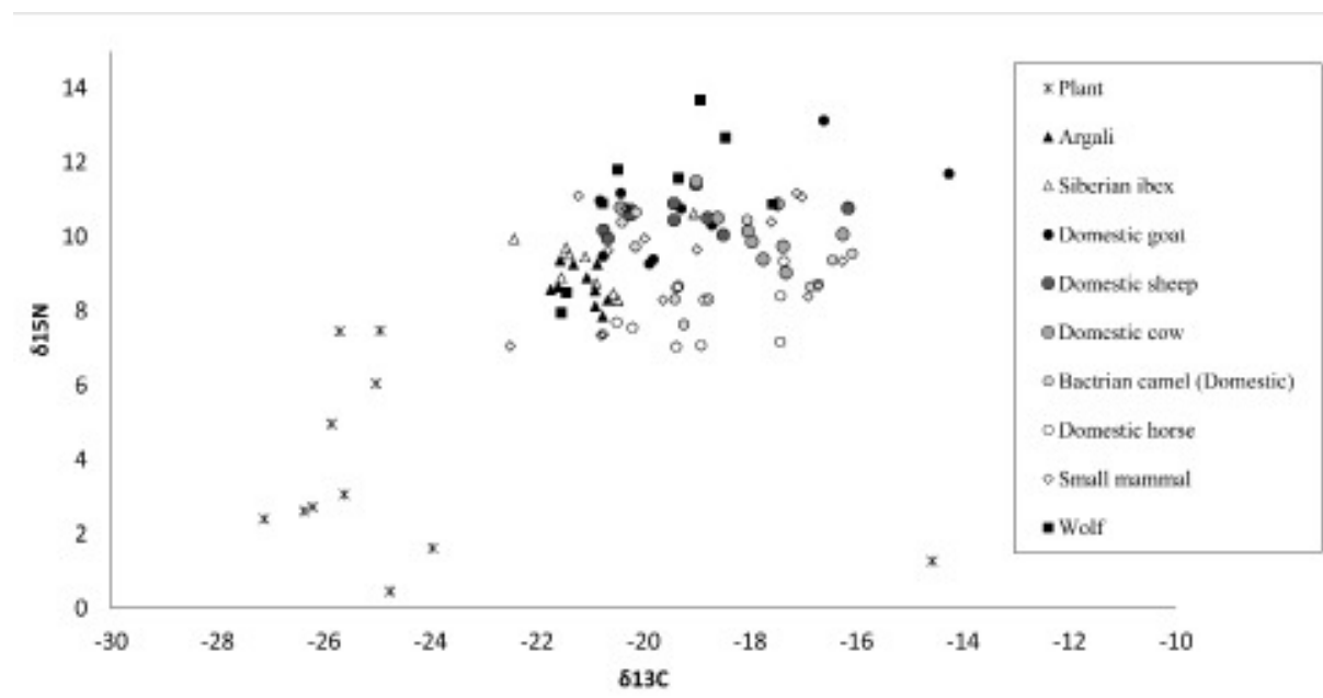
Figure 2. Distribution of plant, wild and domestic ungulate, small mammal, and wolf \delta^{13}\text{C} and \delta^{15}\text{N} values from Ikh Nart Nature Reserve, Mongolia. Plant and small mammal values represent \delta^{13}\text{C} and \delta^{15}\text{N} values for one bulked sample ( N = 3 to 10 individuals) for each species.
