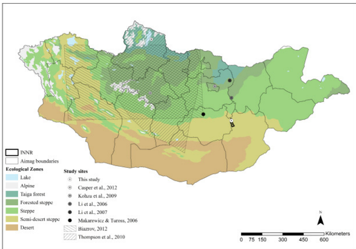
Figure 1. Locations of previous plant and mammal isotope studies in Mongolia, including Ikh Nart Nature Reserve (INNR). Locations presented as points for studies that occurred at small scales, and larger polygons for studies that covered broader areas.
